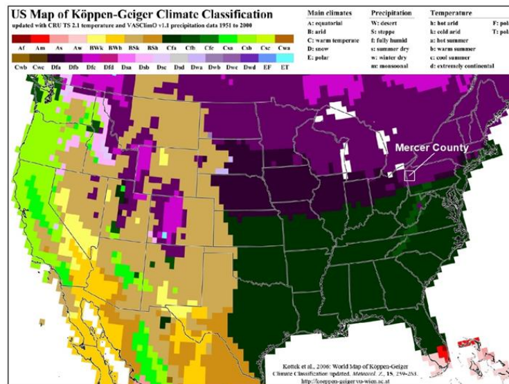
Figure 1 - Köppen-Geiger Climate Map
