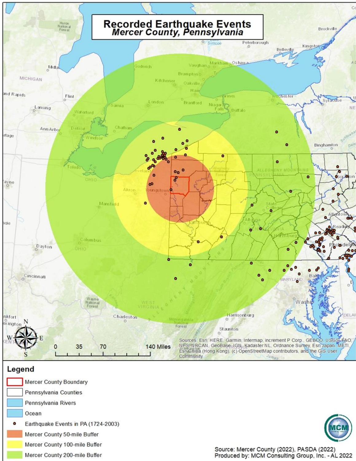
Figure 15 - Pennsylvania Earthquake Activity
